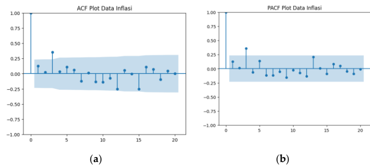
Figure 2. ACF and PACF Plots
